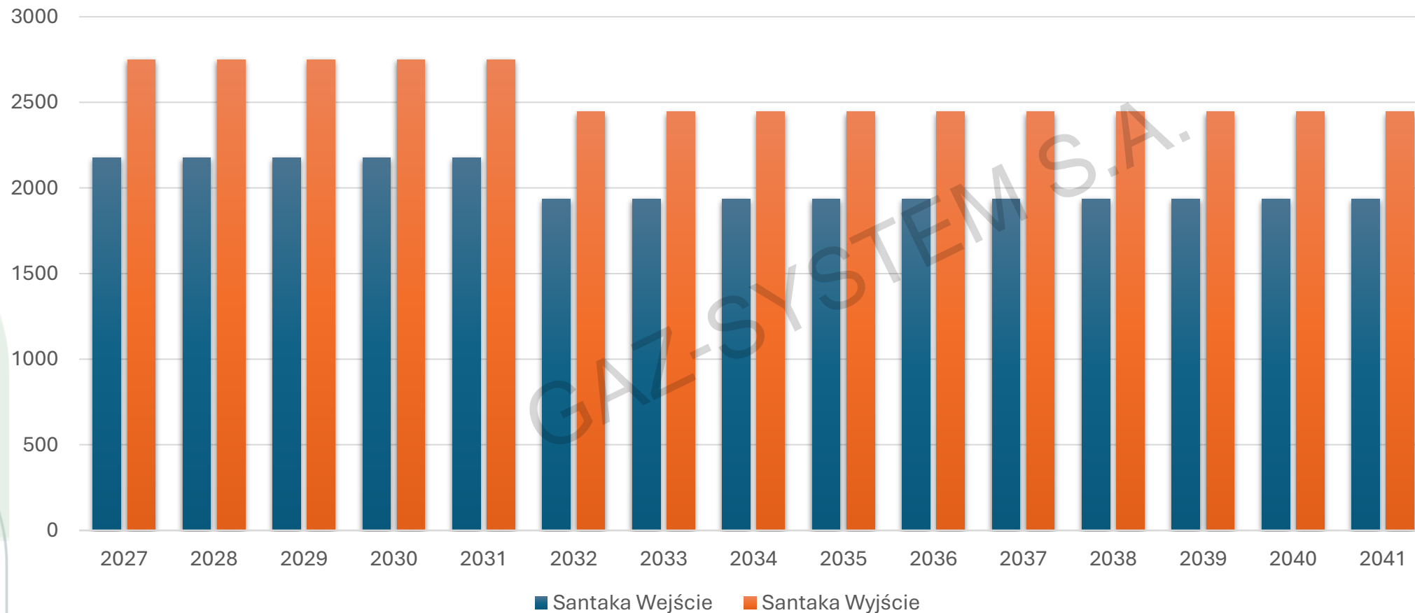
Santaka (PL-LT) [MWh/h]
